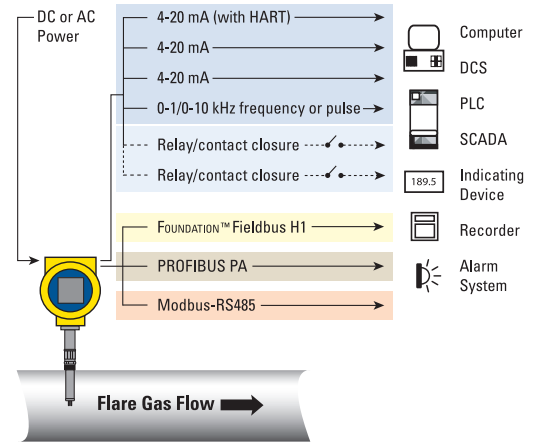
Figure 5: Readouts & Digital Communication
