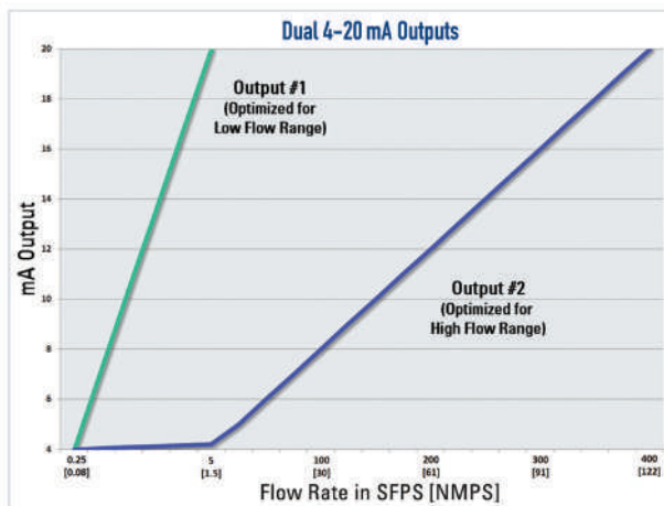
Figure 3: Dual Calibration Performance
