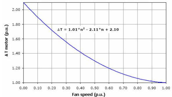
Fig. 6 – Temperature rise x fan speed at rated load
